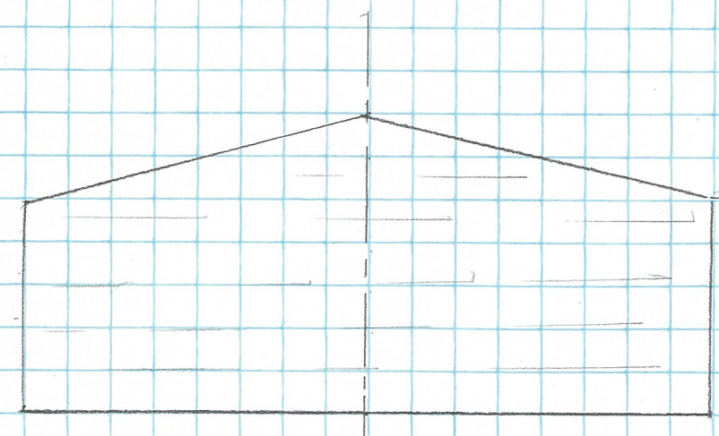
Stabilizer - 1/32 Balsa note: grain is horizontal
